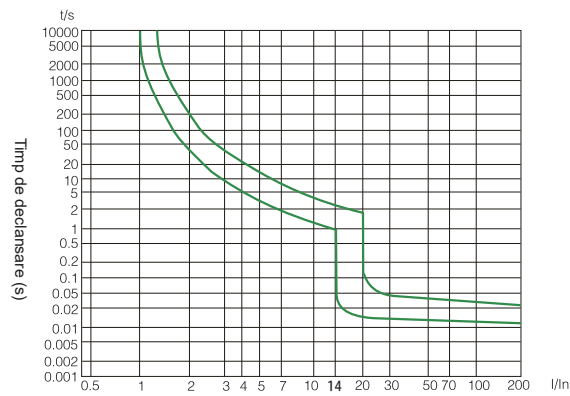
Caracteristica K
